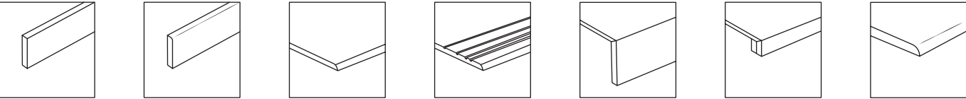
Rodapié cortado Short skirting board Rodapié romado Rounded skirting board Peldaño Romo (sin ranuras) Rounded stair tread (no grooves) Peldaño Romo (ranurado) Rounded stair tread (with grooves) Peldaño Tabica Riser stair tread Peldaño Gradone Gradone stair tread Peldaño Classic Gradone stair tread
