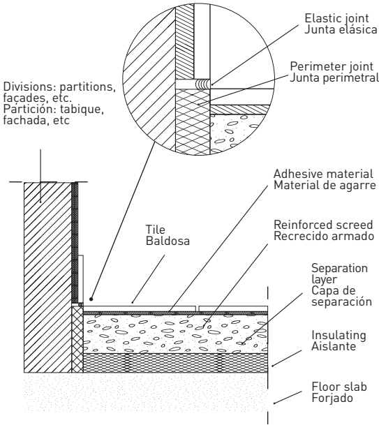
Detail of perimeter joint with sealant | Detalle de junta perimetral con sellante (UNE 138002:2017)
